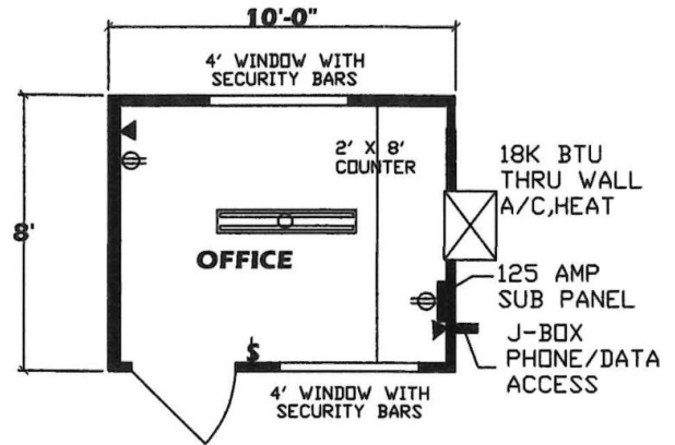
10' OFFICE UNIT
